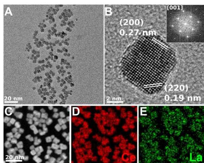
Figure 5 CTEM, AC-HRTEM, HAADF-AC-STEM, and AC-STEM-EDS mapping of the nominal 7.5 mol% La-doped CeO 2 nanocubes. (A) CTEM image showing clusters of La-doped CeO 2 nanocubes. (B) AC-HRTEM image showing a single crystalline La-doped CeO 2 nanocube projected along the [001] zone axis, with the d-spacings for the (200) and (220) lattice planes being shown. Inset shows the corresponding 2D-FFT. (C) HAADF-AC-STEM image of the same nanocubes, showing the scan region imaged for EDS mapping. (D,E) EDS maps showing the distribution of Ce and La throughout the nanocubes, respectively. The EDS overall quantification indicates a molar percentage of Ce and La of 94.5% and 5.5%, respectively.
