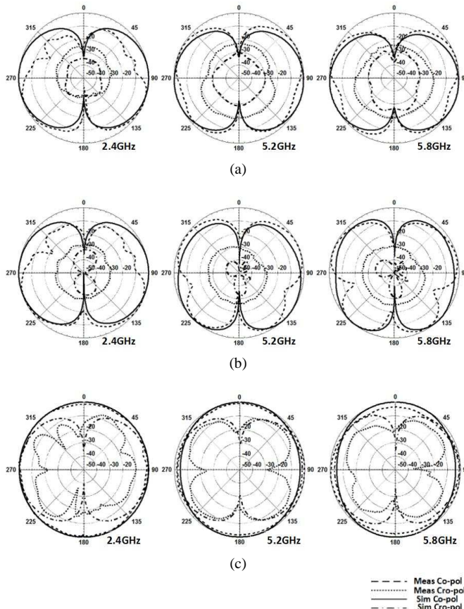
Fig. 20. Radiation patterns (a) at xz plane (b) at yz plane (c) at xy plane.
