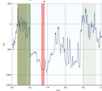
Fig. 16. Surface profile in the CPW transmission line.
