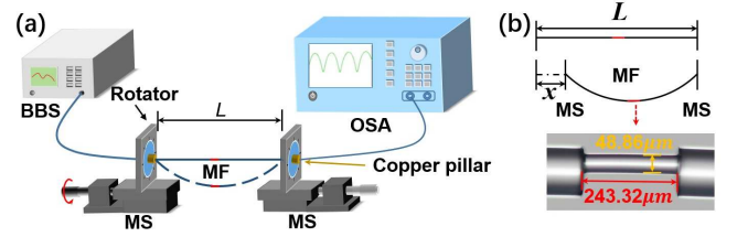
Fig. 2. (a) Experimental setup of the MAMZI-based vector bending sensing system. (b) Sketch for curvature calculation.
