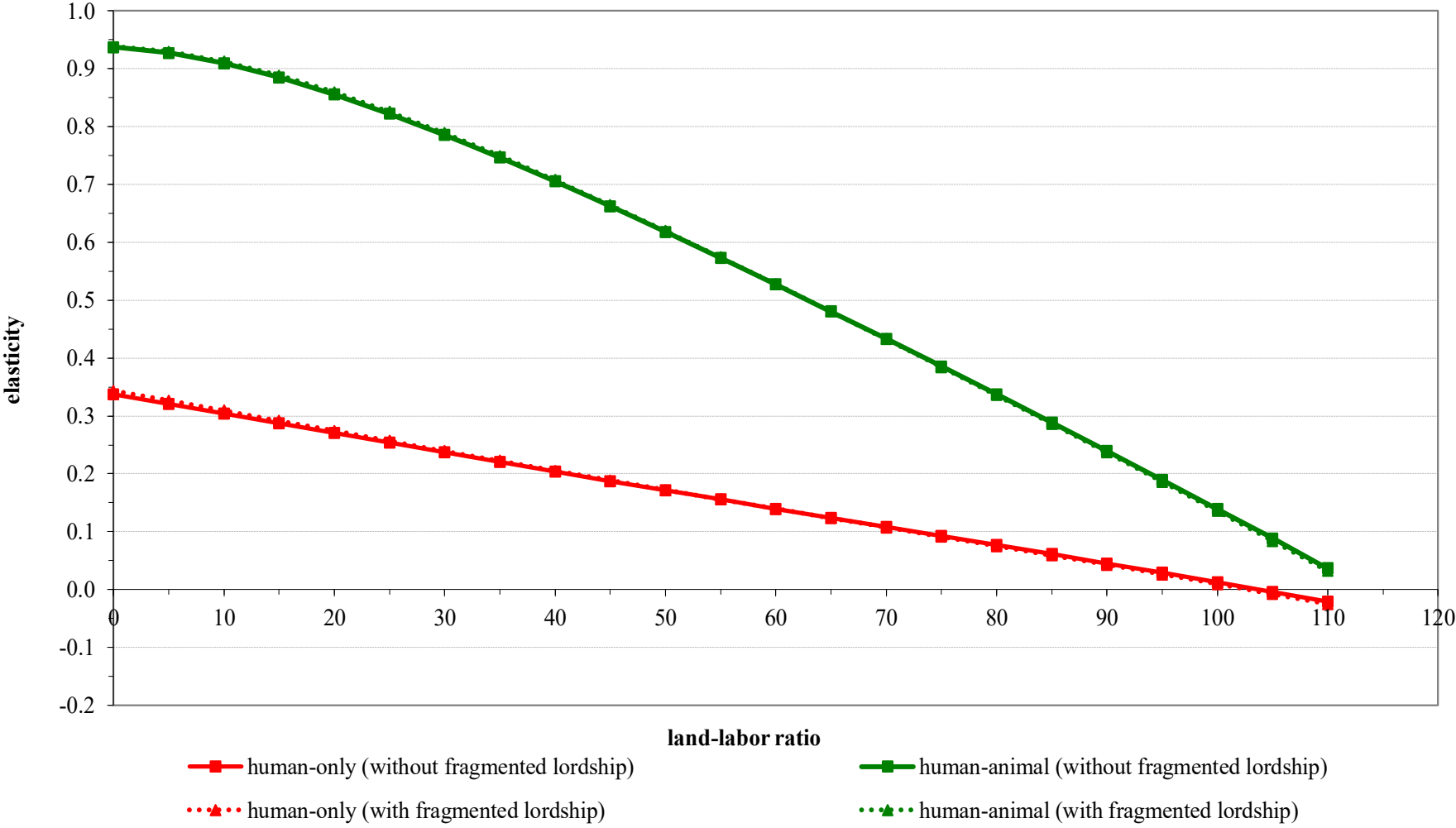
Figure A3: Elasticity of Coerced Labor with Respect to the Land-Labor Ratio, With and Without Fragmented Lordship Dummy, Two-Part Estimates, Bohemia 1757
