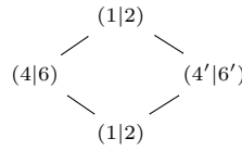
FIGURE 3. The non-simple direct summand of the core of T(8|9) .
