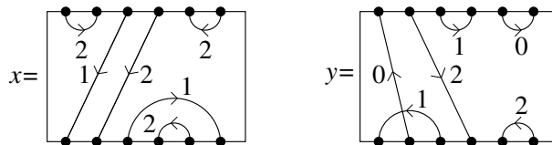
FIGURE 1. Two elements in B_6^3(\delta) .
