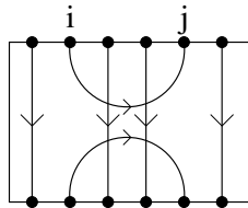
FIGURE 5. The element e_{i,j} .
