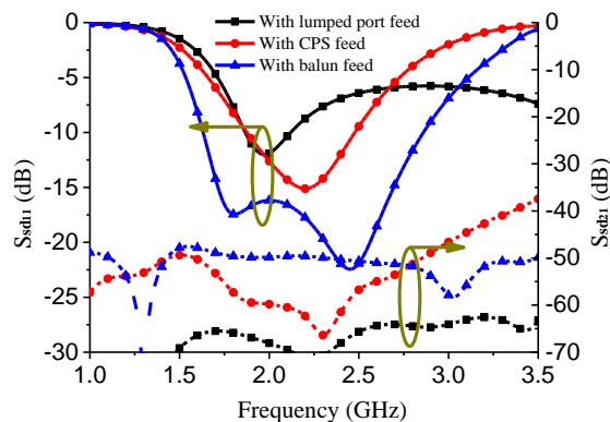
Fig. 11. Simulated S-parameters of the four-port DPSD antenna with different feed methods.
