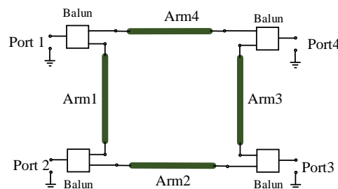
Fig. 9. Equivalent circuit model of the four-port DPSD antenna.
