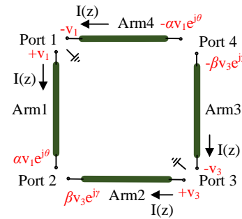
Fig. 2. Equivalent circuit for the DPSD antenna.
