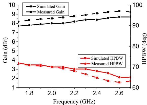
Fig. 24. Simulated and measured gain and HPBW of the highly integrated DPSD antenna for H-plane with the feed point 1 excited.
