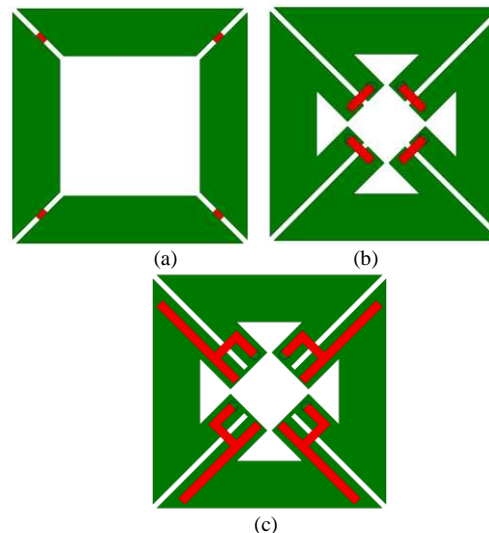
Fig. 10. Design steps of the four-port DPSD antenna. (a) With ideal lumped port feed. (b) With CPS feed. (c) With balun feed.
