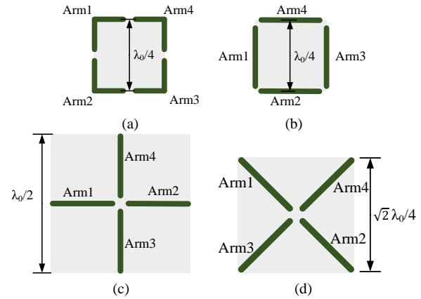
Fig. 1. Different configurations for dual-polarized antenna. (a) \pm 45^\circ polarized DPSD antenna. (b) Horizontal and vertical polarized DPSD antenna. (c) Horizontal and vertical polarized CD antenna. (d) \pm 45^\circ polarized CD antenna.
