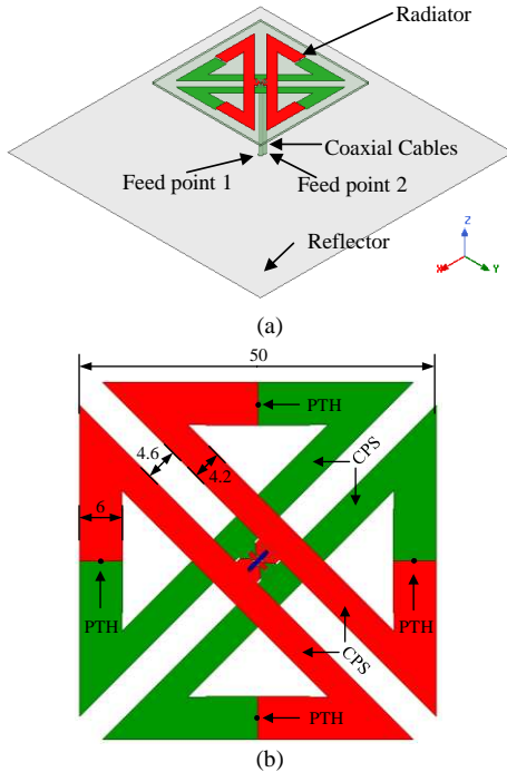
Fig. 19. Geometry of the highly integrated DPSD Antenna. (a) 3D view. (b) Top view of the radiator. (Unit: mm)
