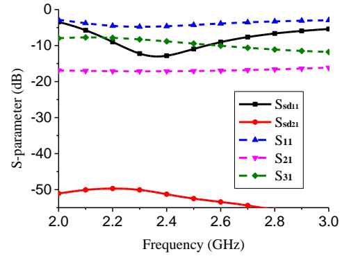
Fig. 7. Simulated S-parameters of DPSD antenna.
