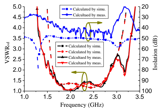
Fig. 14. The calculated VSWR and isolation by the simulated and measured results for the four-port DPSD antenna without feed network.
