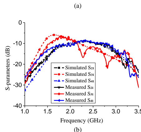
Fig. 13 Simulated and measured S-parameters for the four-port DPSD antenna. (a) S_{11} and S_{22} . (b) S_{21} , S_{31} and S_{41} .
