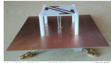
Fig. 21. Photograph of the fabricated highly integrated DPSD antenna.
