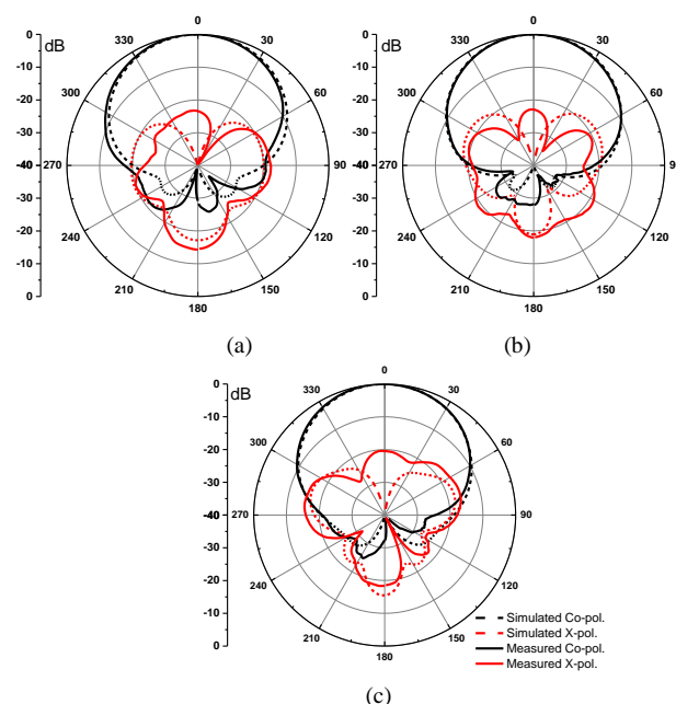
Fig. 17 Simulated and measured radiation patterns of the four-port DPSD antenna with the feed network for the H-plane when the feed point 1 excited. (a) 1.7 GHz. (b) 2.2 GHz. (c) 2.7 GHz.
