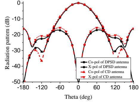
Fig. 6. H-plane radiation patterns of the DPSD antenna and CD antenna.
