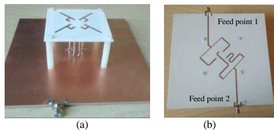
Fig. 15. Photographs of the fabricated four-port DPSD antenna with the feed network. (a) Antenna radiator and reflector. (b) The feed network on the bottom layer of the reflector.
