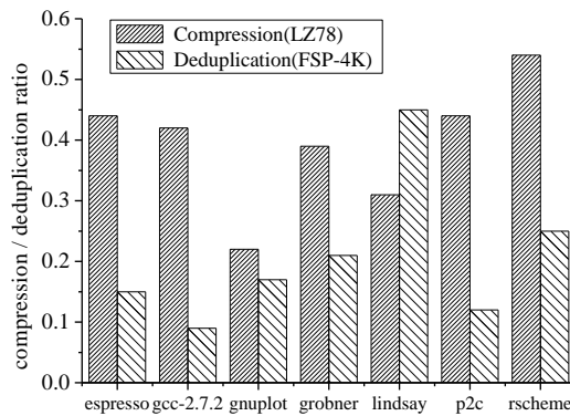
(c) Compression ratio against deduplication ratio
