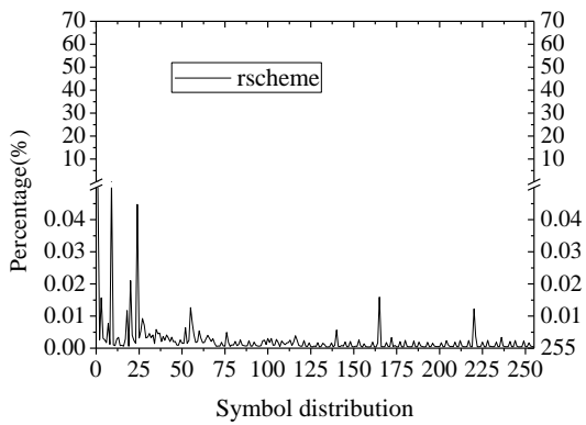
Fig. 3 Symbol distribution of seven traces
