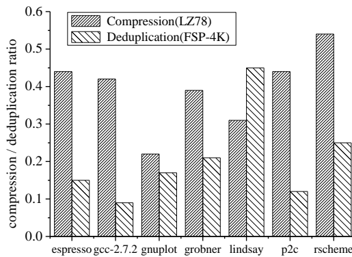
(c) Compression ratio against deduplication ratio Fig.9 Comparison of memory compression and deduplication
