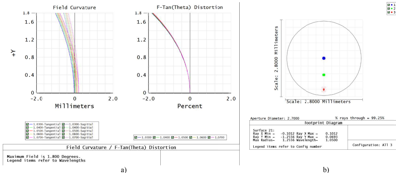
Figure 6. a) Field curvature in the image plane. The maximum field curvature is just under 1 mm at the edge of the field (corresponding to a +Y value of 1.8); b) Footprint diagram of beams corresponding to each the three configurations striking the image plane. The edge of the field is situated at a distance of 1.135 mm from the centre of the field.
