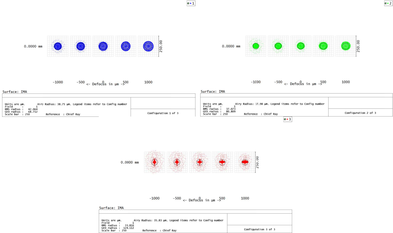
Figure 5. Through focus spot size analysis for each of Configurations 1, 2 and 3. Defocus is modelled over a total distance of 2 mm (1 mm away in either direction from the axial position of the image plane)
