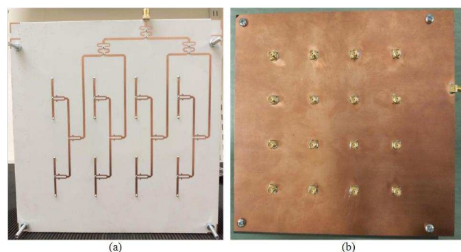
Fig. 9. 1:16 Wilkinson power divider network prototype: (a) top view, (b) bottom view (ground plane with 16 coaxial connectors).
