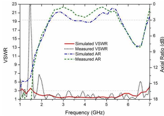
Fig. 10. Simulated and measured VSWR.
