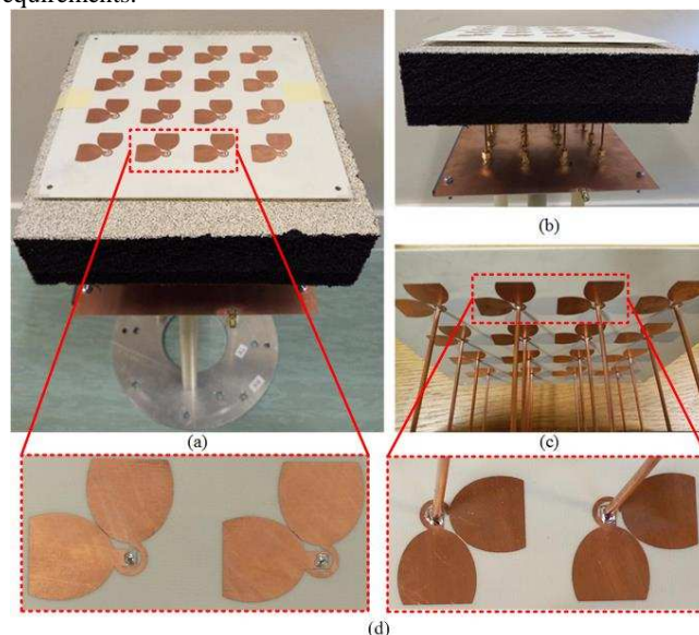
Fig. 8. 4x4 CP-TCCDA prototype: (a) front view, (b) side view, (c) bottom view, (d) feeding details.
