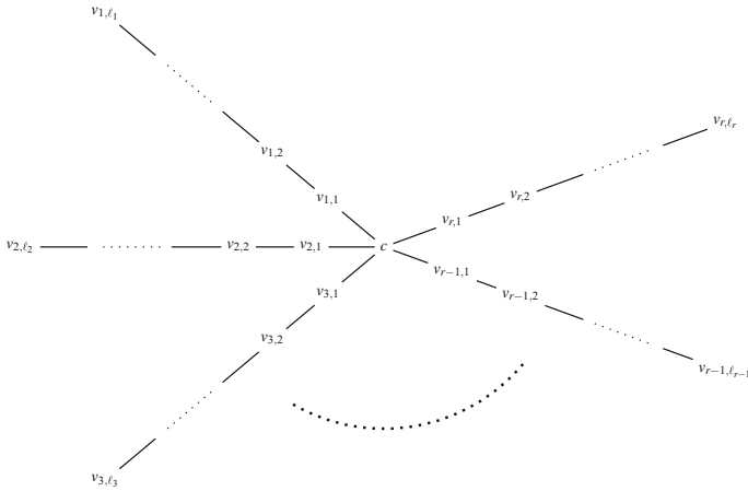
Fig. 3 Star-shaped undirected graph
