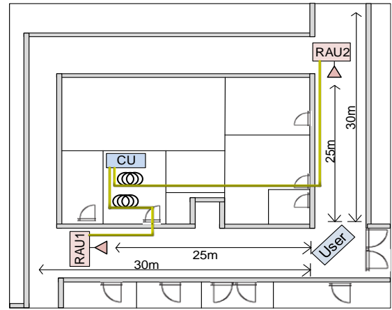
Fig 10. Layout of the Measurement Location
