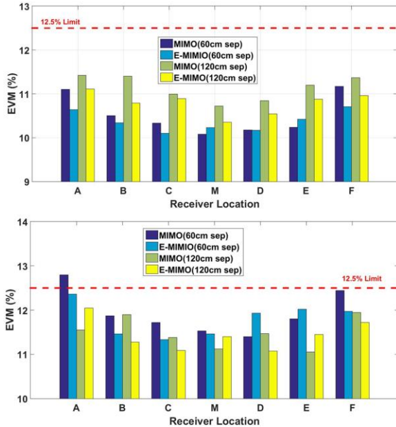
Fig 9. EVM comparison of 2x2 MIMO using STBC processing at 6m (top) and 8m transmission distance (bottom) and equivalent emulated measurements
