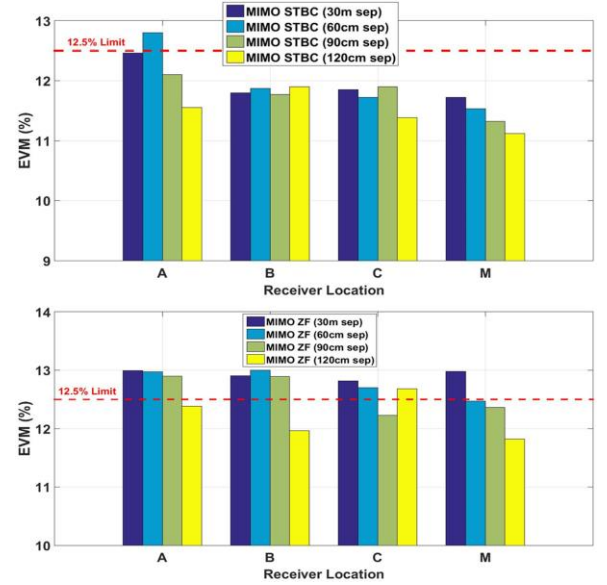
Fig 7. EVM comparison of 2x2 MIMO for various Transmit antenna separation at 8m transmission distance using (upper) STBC (lower) ZF processing
