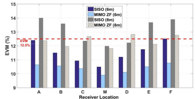
Fig 5. EVM comparison of SISO (0.5Gb/s) versus Zero Forcing MIMO processing (1Gb/s) for 6m (RAU spacing: 60cm) and 8m (RAU spacing: 120cm)
