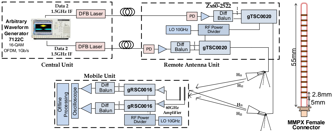
Fig 2. System architecture for the RoF transported 60GHz Distributed MIMO transmission (left) 15dBi Gain Quasi-discooidal slot-array antenna (right)
