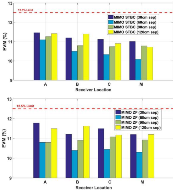
Fig 6. EVM comparison of 2x2 MIMO for various Transmit antenna separation at 6m transmission distance using STBC (upper) and ZF (lower) processing
