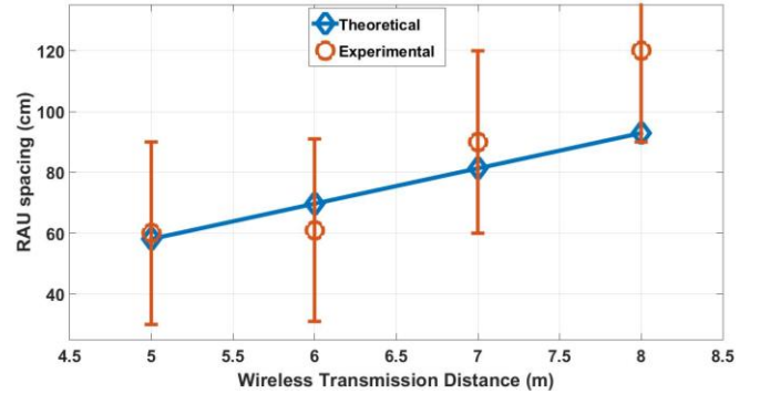
Fig 8. Theoretical Optimum Antenna Spacing for 2x2 MIMO versus Experimental values with error bars to represent the ranges between discrete points at which measurements were taken.
