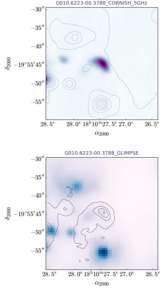
Fig. 2: CORNISH (top panel) and GLIMPSE (bottom panel) images of G010.6223–00.3788, presented as in Fig. 1, with overplotted 8 micron and 6 cm contours, respectively. A dust lane is hiding the source in the 8 micron image.
