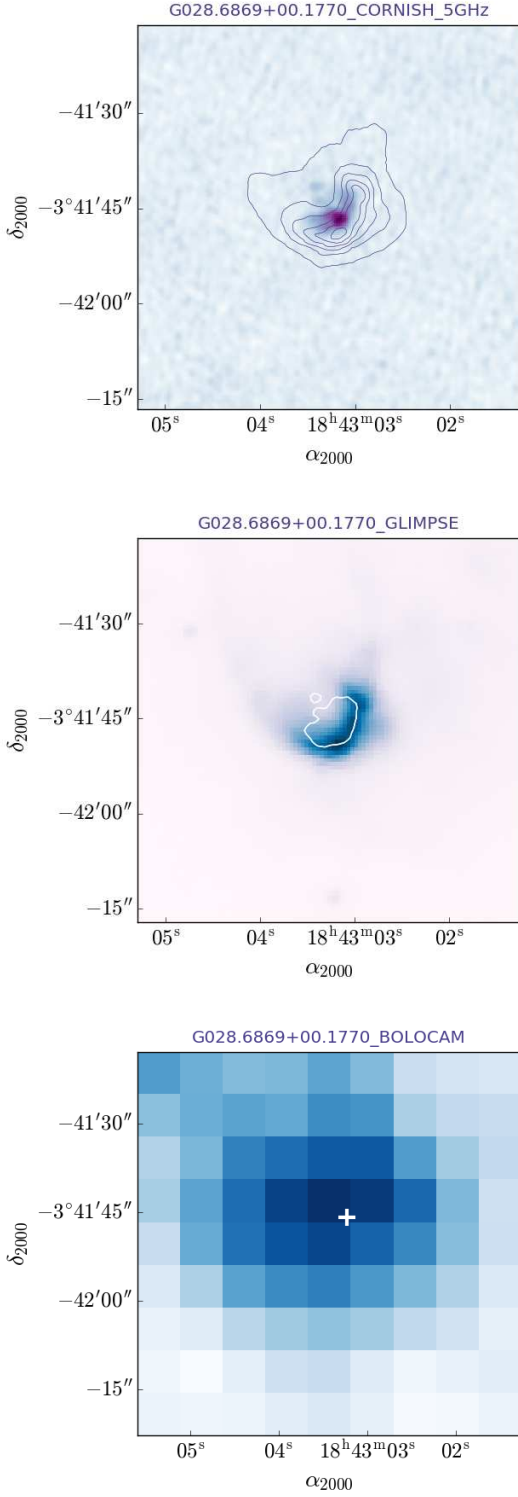
Fig. 1: Images of the cometary UCHII G028.6869+00.1770. Top: CORNISH 6 cm image with overplotted GLIMPSE 8 micron contours, with the corresponding GLIMPSE image shown below, with overplotted radio contours. The morphology at both wavelengths is in very good agreement, and there is excellent positional coincidence between the two catalogues, allowing reliable source identification. The BOLOCAM image (bottom panel) shows a bright unresolved source at 1.1 mm coincident with G028.6869+00.1770 (the source position is marked by a white cross).
