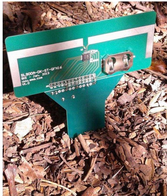
Figure 8. Example of the Soil Stick Sensor for Humidity in a real situation.
