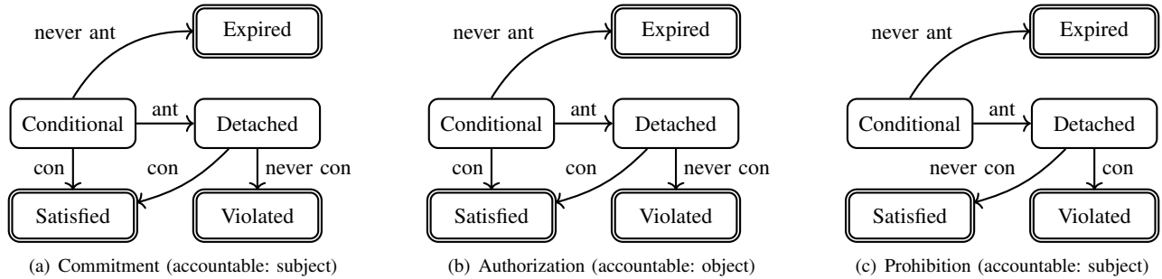
Fig. 1. Lifecycle of norms. Double rectangles represent terminal states (i.e., the norm’s lifecycle ends in those states). To highlight the differences, we use the same layout of states in each diagram.
