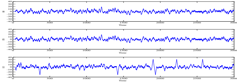
Fig. 10. The plot of the cross-correlation function for 32-bits (a) x xcorr y (b) x xcorr z and (c) x corr z .
