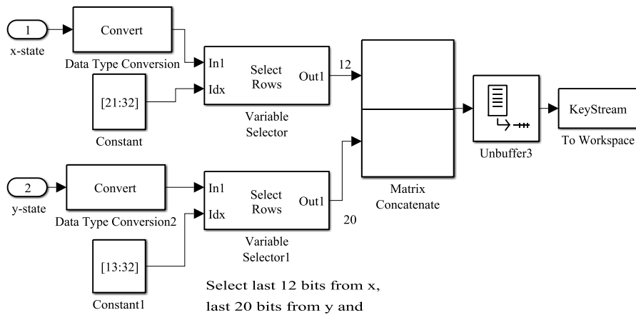
Fig. 5. Scrambling scheme of the Lorenz signals.
