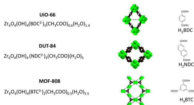
Figure 1. Formula units and graphical representations of the activated zirconium MOFs.
