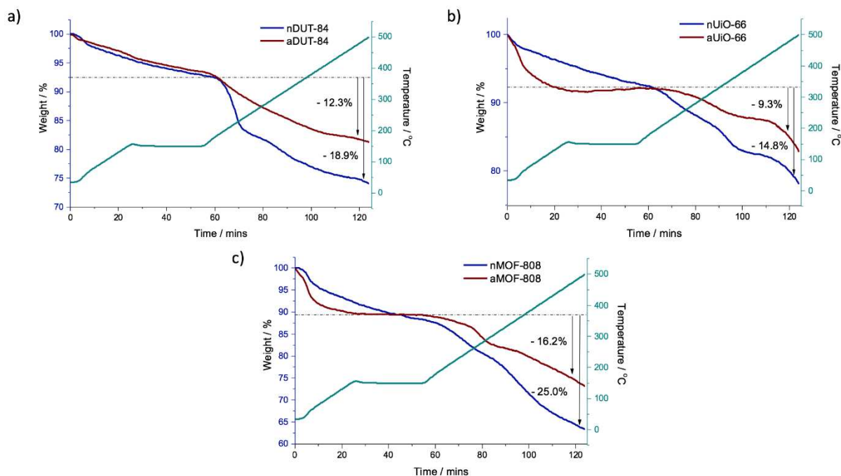
Figure 3. TGA trace for the non-activated and activated counterparts of each MOF. Heating rate: 5\text{ }^{\circ}\text{C min}^{-1} in \text{N}_2 , 30 min isotherm at 150\text{ }^{\circ}\text{C} followed by a ramp to 500\text{ }^{\circ}\text{C} . A value for the % weight loss post isotherm until end of the final ramp is shown on the TGA trace for each material.
