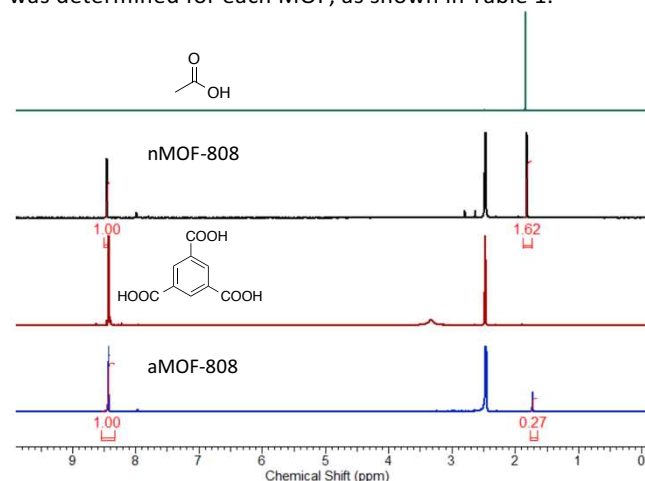
Figure 2. A 1 H NMR (in DMSO/D 2 SO 4 ) overlay showing acetic acid (green), digested nMOF-808 (black), free BTC ligand (red) and the digested aMOF-808 (blue).
