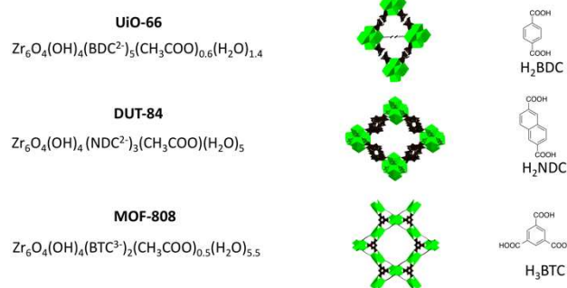
Figure 1. Formula units and graphical representations of the activated zirconium MOFs.
