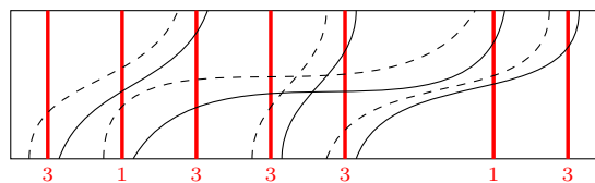
FIGURE 33. The basis element B_S in Example 5.3.
