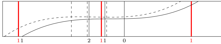
FIGURE 15. Image of the diagram in Figure 13 under \Phi , as in Example 4.10.
