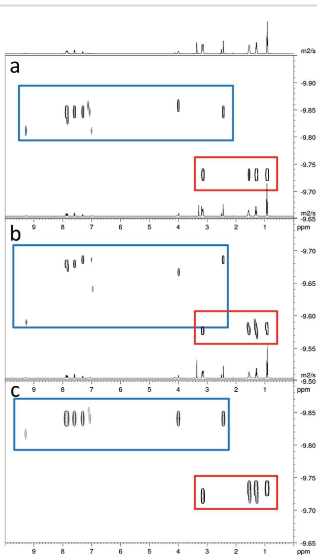
Fig. 12 ^1\text{H} DOSY of 4 (55.56 mM) in \text{DMSO-}d_6 (a) 26.15 °C; (b) after heating to 38.65 °C; (c) when cooled back to 25.95 °C. Anionic component of 4 is highlighted in blue, TBA counter cation has been highlighted in red.
