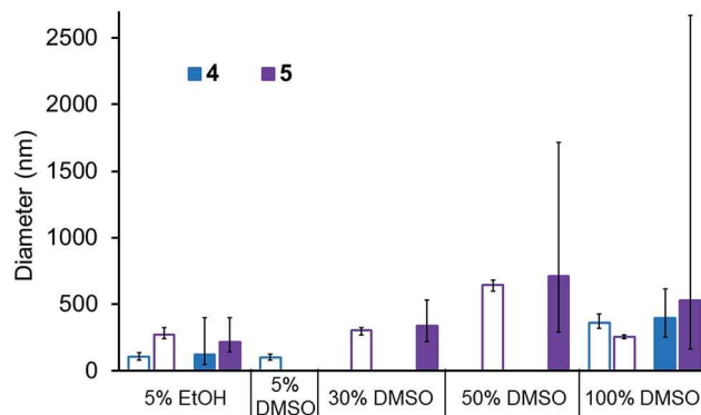
Fig. 10 Bar chart comparing the peak maxima obtained from DLS (filled bars) average intensity size distribution studies in a range of aqueous solutions of 4 (0.56 mM) and 5 (0.56 mM) with the average size of structures observed in microscopy images (unfilled bars) of 4 (0.50 mM) and 5 (0.50 mM) in the same range of aqueous solutions. The error bars give the full range of aggregate sizes, comparing the peak widths obtained from DLS average intensity size distribution and microscopy studies.
