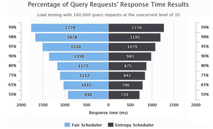
Fig. 9. Experiment 2: Percentage of the service requests served within a certain time (Million Seconds)
