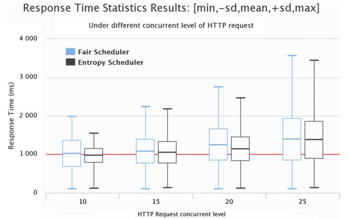
Fig. 6. Experiment 1: Statistics result for service response time
