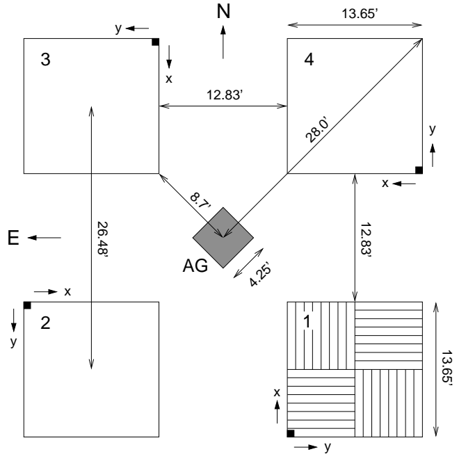
Figure 1. The WFCAM focal plane showing the four detectors and the autoguider (AG). Numbering of detectors is the same as that used in the WSA and for extension numbering in the multi-extension FITS image files. Detectors are divided into four quadrants, each quadrant having 8 channels as illustrated in detector 1. Note the convention used for the image pixel co-ordinate system in each detector. In this figure taken from Dye et al. (2006), north is upwards and east is to the left.
