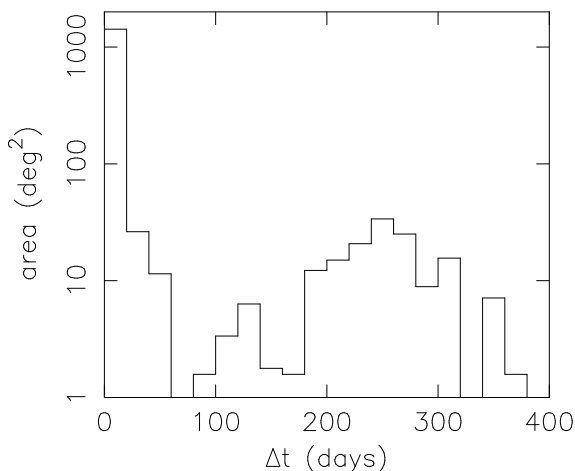
Figure 5. Areal coverage of repeats in this release binned by the time elapsed between the first and last observation within a group of repeat observations. This amounts to a total area of \sim 1630 \text{ deg}^2 and has been computed for all data in the release, including data that have not passed QC but are included in the extended release. Within this, an area of approximately 1410 \text{ deg}^2 has repeat imaging where at least two of a group of repeats pass QC.
