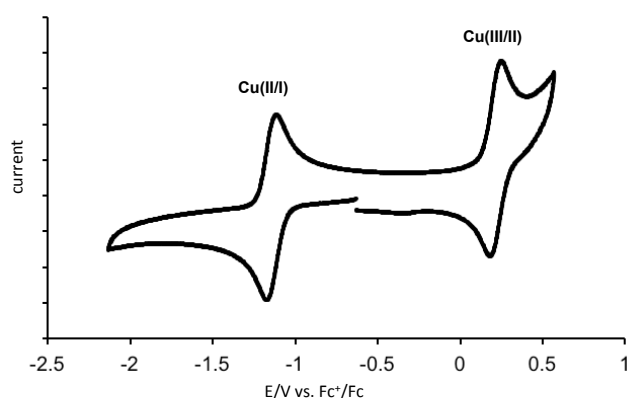
Fig. 3. Exemplar cyclic voltammogram of Cu(30) in deoxygenated anhydrous DMSO/0.1 M [Bu 4 N][BF 4 ] at 0.1 V/s scan rate.
