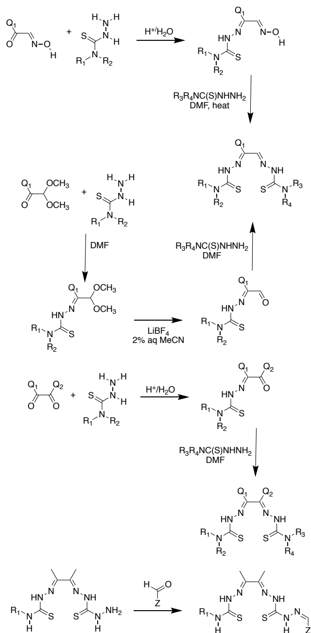
Fig. 2. Literature routes for synthesis of dissymmetric bis(thiosemicarbazone) pro-ligands using isonitronne or acetal protection and using unprotected diketones, and dissymmetric functionalisation via a thiocarbohydrazide side arm.
