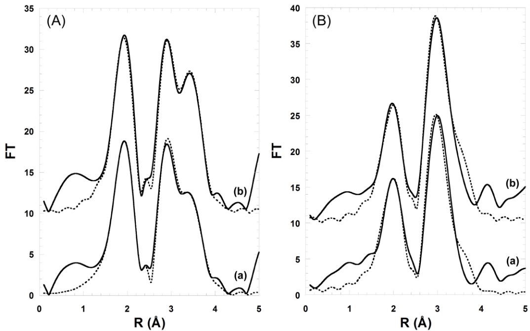
Figure 5. Phase shift corrected Fourier transforms of k^3\chi(k) spectra at the Co K-edge (A) and Ni K-edge (B) from experiment (—) and fit results (···): (a) AERO_NiCo 2 O 4 ; (b) BULK.
