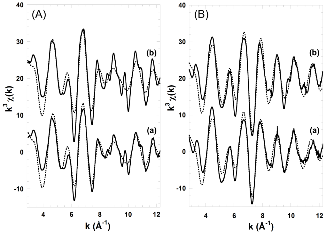
Figure 4. k^3\chi(k) at the Co K-edge (A) and Ni K-edge (B) from experiment (—) and fit results (···): (a) AERO_NiCo 2 O 4 aerogel; (b) BULK.
