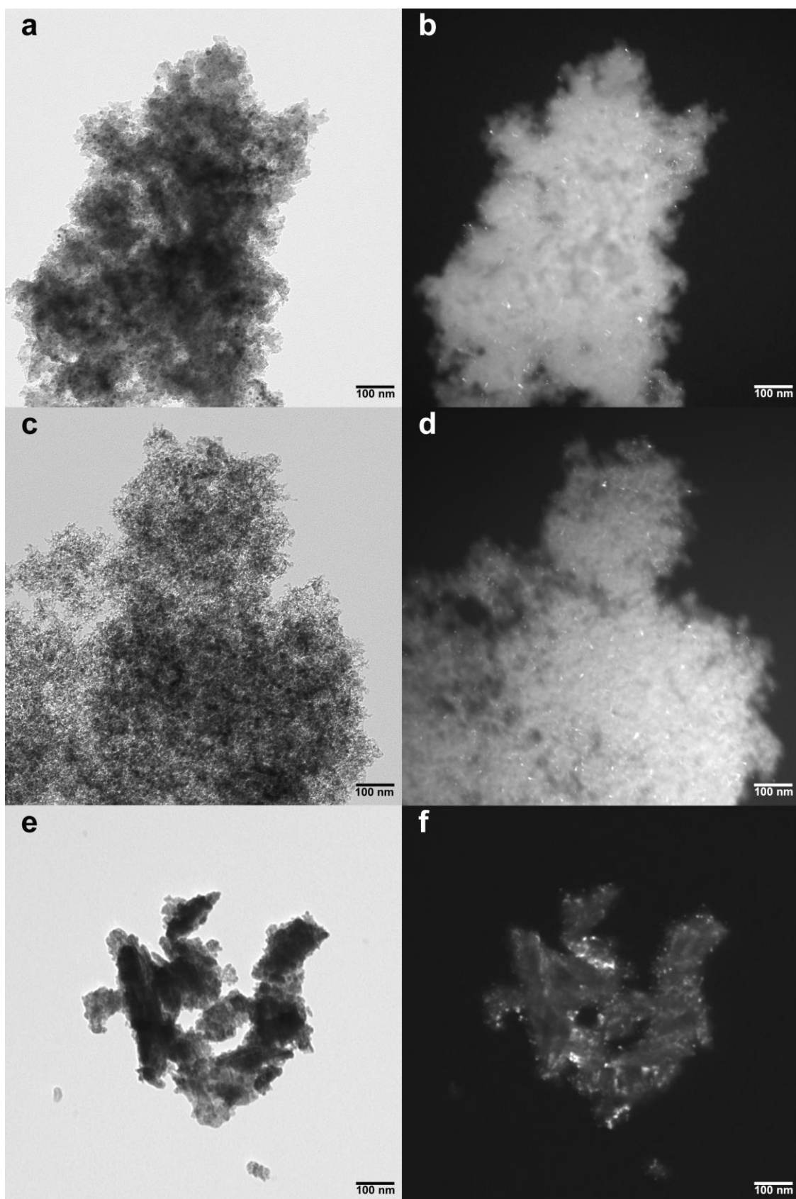
Figure 2. BF (left) and DF (right) TEM images of the AERO_800red (a,b), AERO_NiCo 2 O 4 (c,d) and BULK (e,f) samples.
