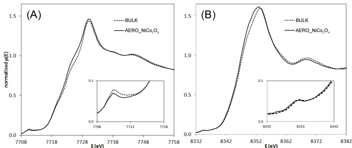
Figure 3. XANES spectra at the Co K-edge (A) and Ni K-edge (B) for AERO_NiCo 2 O 4 and BULK.
