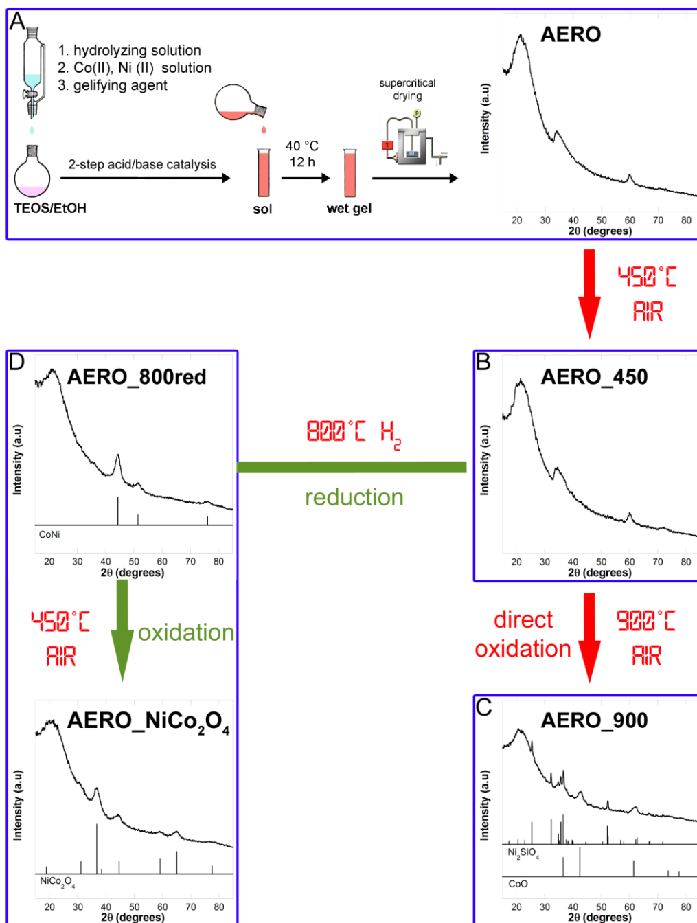
Figure 1. Schematic of the sol-gel method and post synthetic thermal treatments used to obtain a sample made out of nickel cobaltite nanoparticles dispersed in a highly porous silica aerogel matrix.
