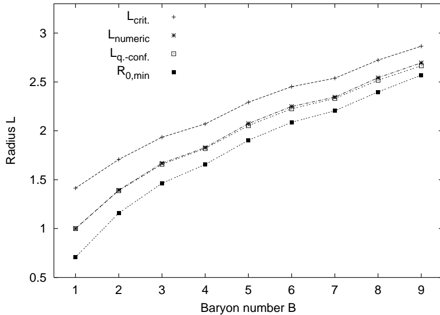
Figure 7: The radii L_{opt.}^{\text{numeric}} , L_{opt.}^{q\text{-conf.}} , L_{\text{crit.}} , and R_{0,\min} as a function of the baryon number B .
