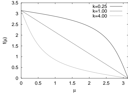
(a) f(\mu) for B = 1
