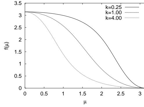
(b) f(\mu) for B = 4
