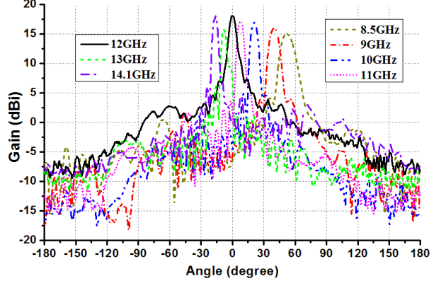
Fig.13 Measured gain patterns of beam steering.
