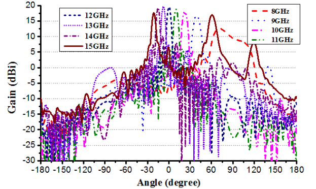
Fig.9 Simulated gain patterns of beam scanning.
