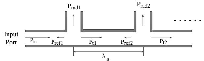
Fig. 4 CTS radiation stub operation principle.
