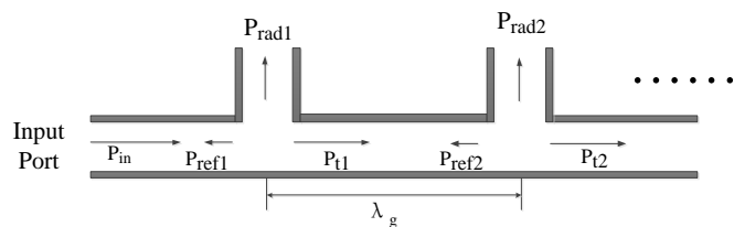
Fig. 4 CTS radiation stub operation principle.
