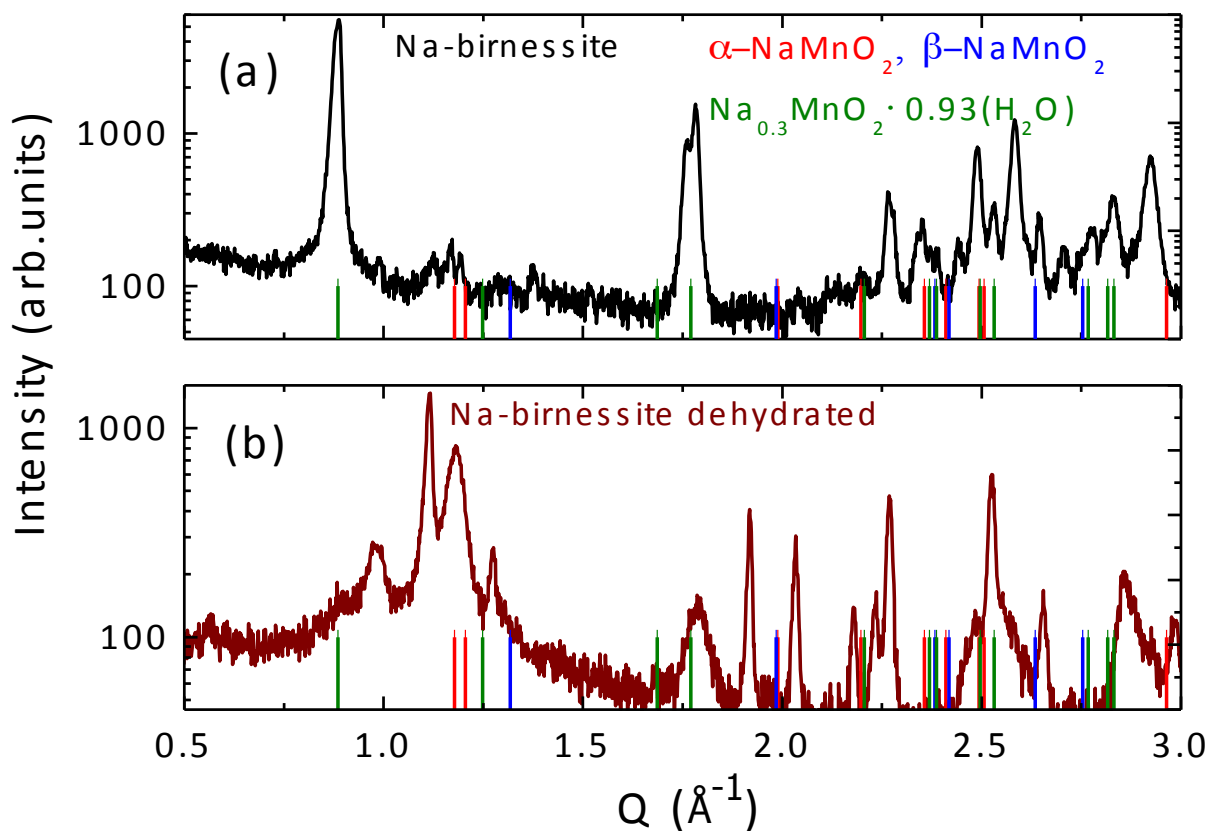
FIG. 6. Comparison of the XRPD patterns of the \text{Na}_{0.3}\text{MnO}_2 \cdot 0.2\text{H}_2\text{O} birnessite's polycrystalline powder (a) and the dehydrated compound (b) taken after the TGA experiment performed up to 1100^\circ\text{C} . Indexing of the reflections has been done on the basis of the \alpha\text{-NaMnO}_2 (ICSD 16270), \beta\text{-NaMnO}_2 (ICSD 16271) and the \text{Na}_{0.3}\text{MnO}_2 \cdot 0.93\text{H}_2\text{O} (ICSD 262208) phases, whose Bragg reflections are indicated with red, blue and green tick marks, respectively. Bragg peaks attributed to the \text{Mn}_3\text{O}_4 (ICSD 68174, ICSD 1514104) are left without tick marks for ease of comparison.
