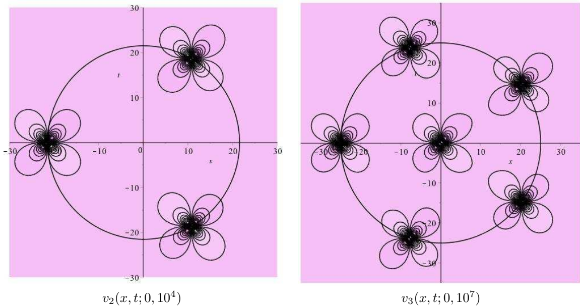
Figure 5.2: Contour plots of the solutions v_2(x, t; 0, 10^4) and v_3(x, t; 0, 10^7) of the Boussinesq system.
