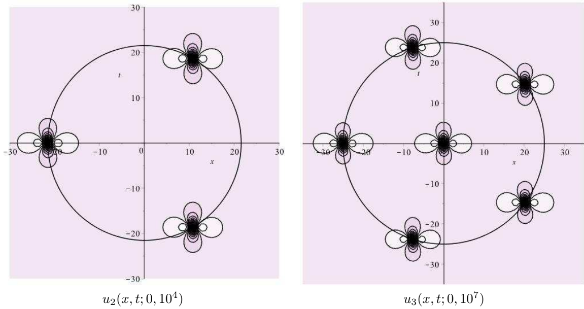
Figure 5.1: Contour plots of the solutions u_2(x, t; 0, 10^4) and u_3(x, t; 0, 10^7) of the Boussinesq equation.
