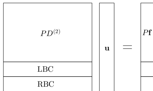
Figure 4: In the alternative approach introduced by Driscoll and Hale, boundary conditions are appended to a rectangular differentiation matrix, where the second-order differential operator D^{(2)} is rectangularized by the barycentric interpolation matrix P and the right hand side \mathbf{f} is mapped to the same grid too.
