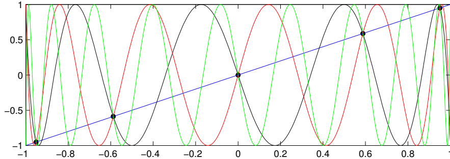
Figure 2: Aliasing of T_1 , -T_9 , -T_{11} , and T_{19} on the 5-point Chebyshev grid of the first kind.
