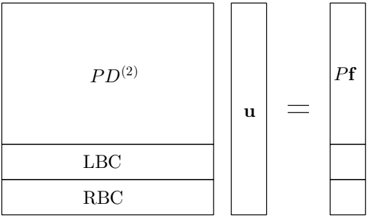
Figure 4: In the alternative approach introduced by Driscoll and Hale, boundary conditions are appended to a rectangular differentiation matrix, where the second-order differential operator D^{(2)} is rectangularized by the barycentric interpolation matrix P and the right hand side \mathbf{f} is mapped to the same grid too.
