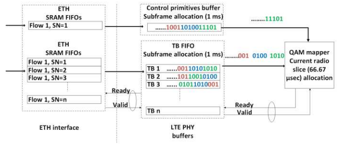
Fig. 2. Control primitives and TB data need to be time aligned at the receiver. SN=Sequence Number, ETH=Ethernet interface, SRAM=Static RAM, FIFO=First-in First-out.
