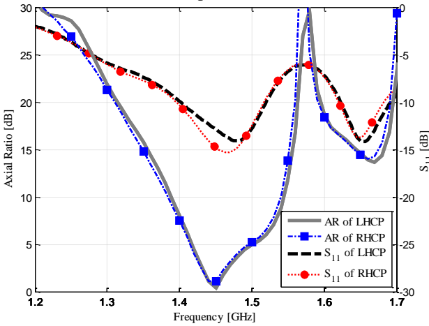
Fig. 8. Switchable capability in terms of AR and S_{11} versus frequency
