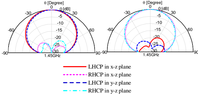
Fig. 9. Switchable capability in terms of radiation patterns
