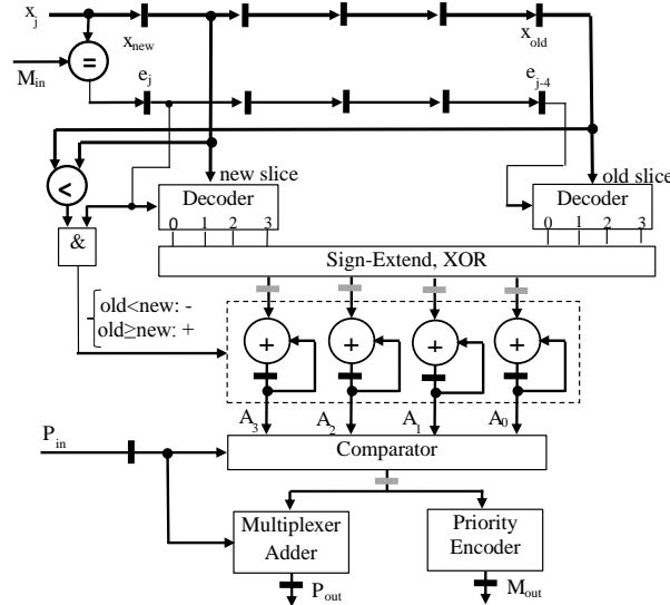
Fig. 1. A front-end block processing 2-bit slices on 5 integers. This block generates 2-bit of the median M_{\text{out}} and the P value ( P_{\text{out}} ) for the next block.
