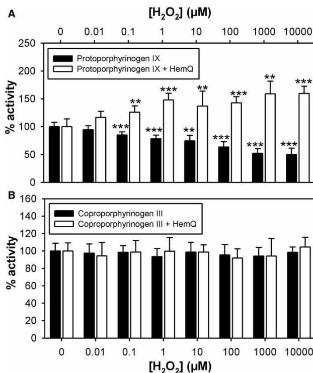
Figure 5. Hydrogen peroxide stimulates protoporphyrinogen oxidase activity in the presence of HemQ.
