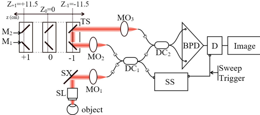
Fig. 2. Schematic diagram of the SS-OCT imaging system used in the present study. SS: swept source; DC1, DC2: directional couplers; BPD: balance photodetector; D: digitizer; MO 1-3 : microscope objectives; TS: translation stage; M 1,2 : flat mirrors; SX: transversal scanner; SL: scanning lens.
