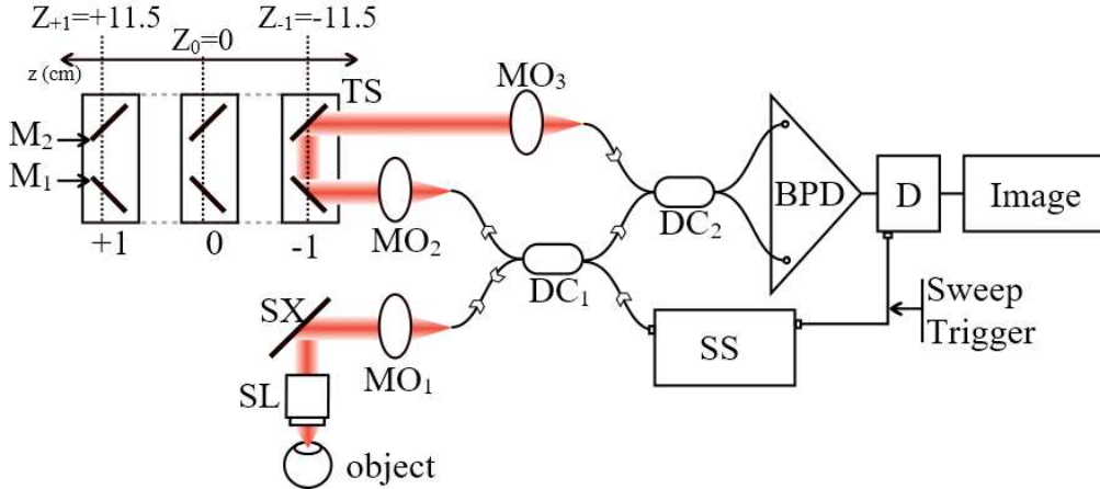
Fig. 2. Schematic diagram of the SS-OCT imaging system used in the present study. SS: swept source; DC1, DC2: directional couplers; BPD: balance photodetector; D: digitizer; MO_{1-3} : microscope objectives; TS: translation stage; M_{1,2} : flat mirrors; SX: transversal scanner; SL: scanning lens.
