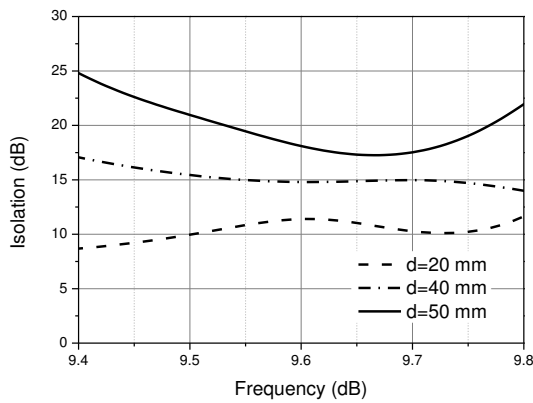
Fig.8. Isolation between inter-elements in FP cavity
