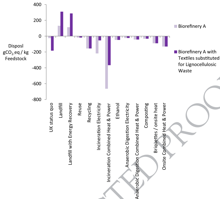
Figure 3 Influence of classifying textiles as lignocellulosic waste.
