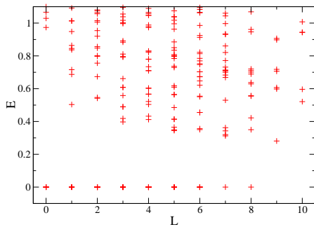
FIG. 2. (color online) Spectrum of the model Hamiltonian (1) for N_\uparrow + N_\downarrow = 4 + 4 on a sphere with N_\phi = 8 flux quanta, i.e., n = 2 flux quanta above the ground state as a function of total angular momentum L . The counting of quasihole states in the zero-energy manifold matches the theoretical prediction given in Eq. (18). We further identify the gap in this finite-size system to be \Delta_{N=8} \simeq 0.2812 .
