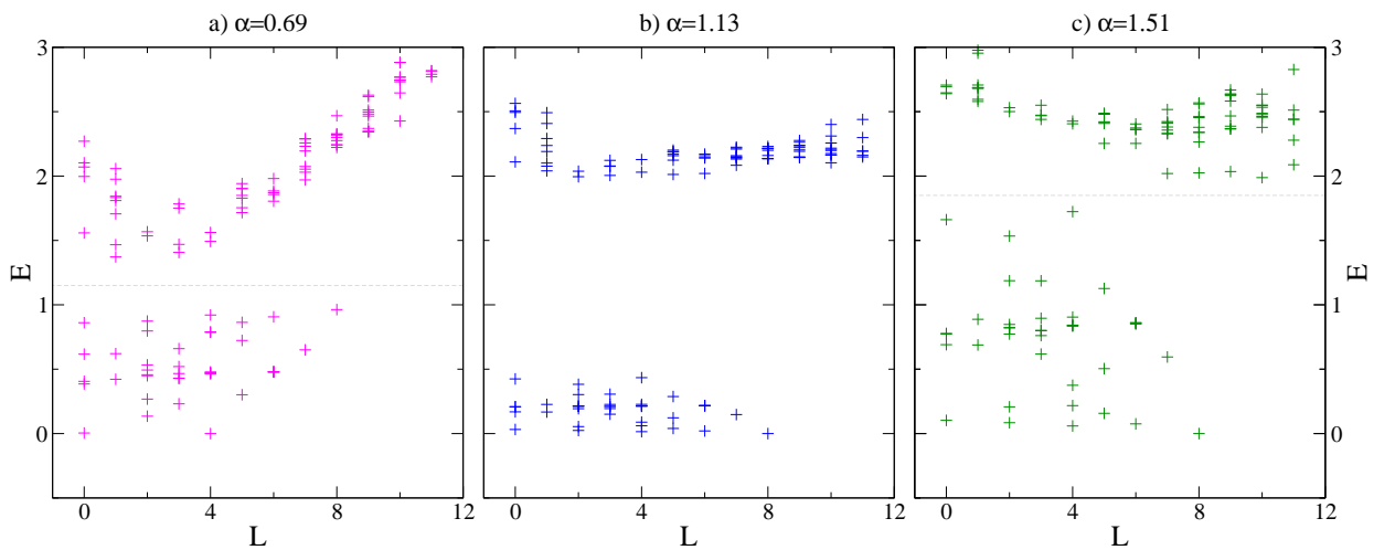
FIG. 4. (color online) Spectrum of the generalized pair tunneling Hamiltonian (13) for N = N_\uparrow + N_\downarrow = 8 on a sphere with N_\phi = 8 flux quanta, i.e., n = 2 flux quanta above the ground state as a function of total angular momentum L . Energies are given in natural units of V_0 , relative to the lowest energy state at each \alpha . Spectra are shown for a) \alpha = 0.22\pi \simeq 0.69 , b) \alpha = 0.36\pi \simeq 1.13 , and c) \alpha = 0.48\pi \simeq 1.51 . For values \alpha \simeq 1 , such as shown in panel b), there is a clear gap. Tuning further away from \alpha = 1 , the quasihole spectrum acquires more dispersion, and finally merges into the continuum of excited states. Panels a) and c) show spectra near the lower and upper boundary of the region in \alpha for which the counting of quasihole states in the low-energy manifold still matches the count of states for \hat{\mathcal{H}}_{220} . Grey dashed lines highlight the separation of the low-energy manifold of states and other excited states.
