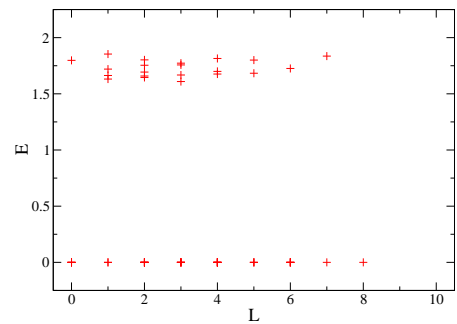
FIG. 3. (color online) Spectrum of the two-body contact interaction in the \uparrow\downarrow basis, \hat{\mathcal{H}}_{220}^{\uparrow\downarrow} , for N = 8 particles on a sphere with N_\phi = 8 flux quanta, i.e., n = 2 flux quanta above the ground state. The Hamiltonian has a large number of zero-energy states, but the degeneracy of this quasihole subspace is found to be lower than the corresponding degeneracy obtained for the case of \hat{\mathcal{H}}_{3-2} . The system features a large gap of \Delta \simeq 1.609 (known to be robust in the thermodynamic limit).
