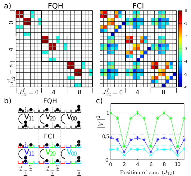
FIG. 2. (a) Magnitudes of matrix elements for the two-body delta interaction between pairs of particles with incoming (outgoing) momenta J_{12}^{i(f)} = [(J_1 + J_2) \text{mod } N_{\text{cell}}] in a finite size geometry for the FQHE on the torus with N_\phi = 12 (left) and for the FCI in the lowest band of the Haldane model for a 3 \times 4 lattice (right). (b) Schematic showing some short range interactions, including a ‘squeezing’ process V_{11} as well as two diagonal interaction terms V_{20}, V_{00} . Panel (c) shows how the magnitude of these processes depends on the centre of mass position for the FCI (solid) as compared to FQH (dashed).
