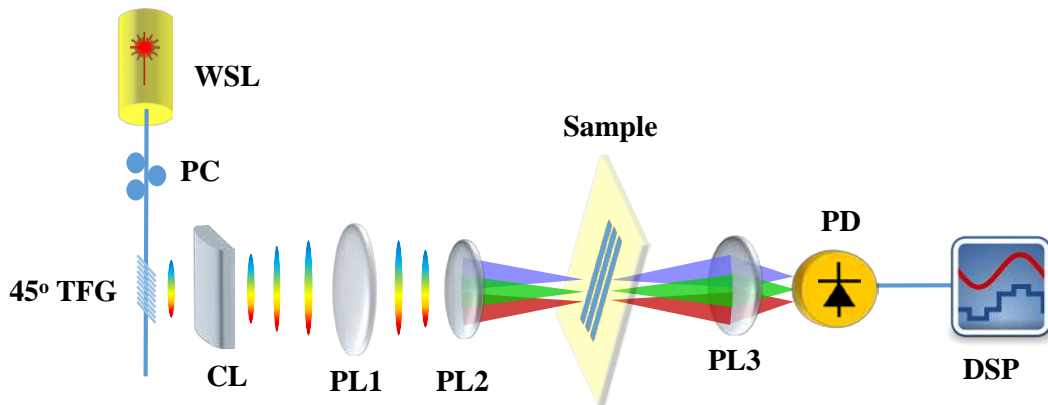
Figure 4. Schematic diagram of the SEI system based on a 45° TFG. WSL: wavelength swept laser, PC: polarization controller, TFG: tilted fiber grating, CL: cylindrical lens, PL: plano-convex lens, PD: photo-detector, DSP: digital signal processing.
