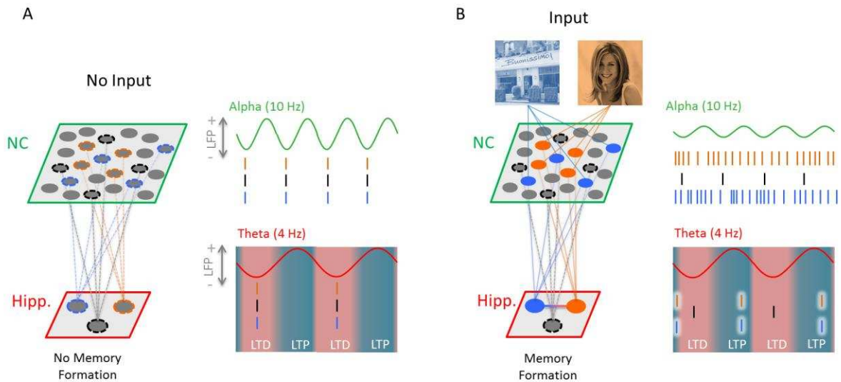
Figure 2. A schematic of the current framework. (A) In the absence of external input, high alpha power is evident in the neocortex (NC), with NC neurons firing at a low rate. In this state, the NC neurons have little impact on their downstream neurons in the hippocampus. LTP/LTD is regulated by the theta phase, whereby in the absence of input, the synaptic connections get weakened (LTD). (B) Input reduces (effective) firing threshold for stimulation-specific populations in the NC which, in this case, respond to two stimuli. On the population level, neuronal firing increases which leads to a decrease in synchrony and alpha power. The increased firing in the two NC populations of neurons would in turn reduce the (effective) firing threshold of their hippocampal stimulation-specific downstream neurons, causing phase precession (indicated by arrows) and hence LTP, which then forms an association between the two stimuli. Note that the phase of theta changes depending on which hippocampal sub-region it is recorded from [29], being 180^\circ phase shifted between the hippocampal fissure and CA1/CA3. We here plot theta as would be recorded in CA1 (and CA3), in keeping with studies that showed LTP to occur at the peak (+) and LTD to occur at the trough (-) of theta [57, 59]. Moreover, as presented here the peak of theta is in fact the functionally inhibitory phase, while its trough is the functionally excitatory phase.
