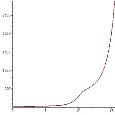
(a) Parametric plot of (z(Z), u(Z)) .
