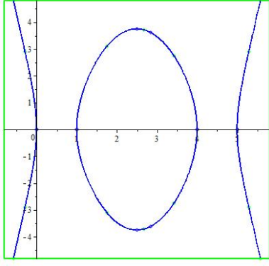
(a) The quartic curve (96) in the (\pi, \pi') plane.
