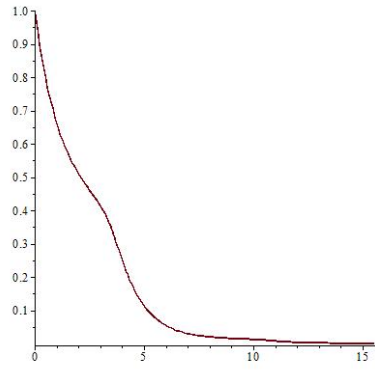
(b) Parametric plot of (z(Z), v(Z)) .
