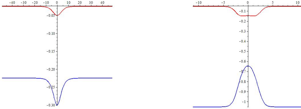
(a) Dark soliton case: k = 1/2 , \delta = 1 , r_0 = 4 with c = 3/4 , C = 1/10 . (b) Bright soliton case: k = 1/2 , \delta = 1 , r_0 = 2 with c = 9\sqrt{10}/20 , C = 1/\sqrt{10} .
