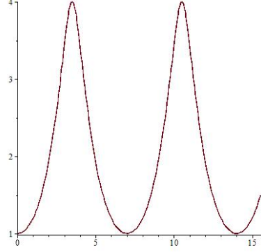
(b) Parametric plot of (z(Z), \pi(Z)) .
