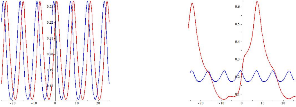
(a) Plots of u and v at t = 0 with \kappa = 1 . (b) Plots of u and v at t = 0 with \kappa = \exp(\sin X) .
