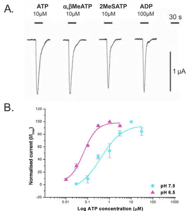
Fig. 5. Pharmacology of the recombinant P2X 2-3/3 receptor.
