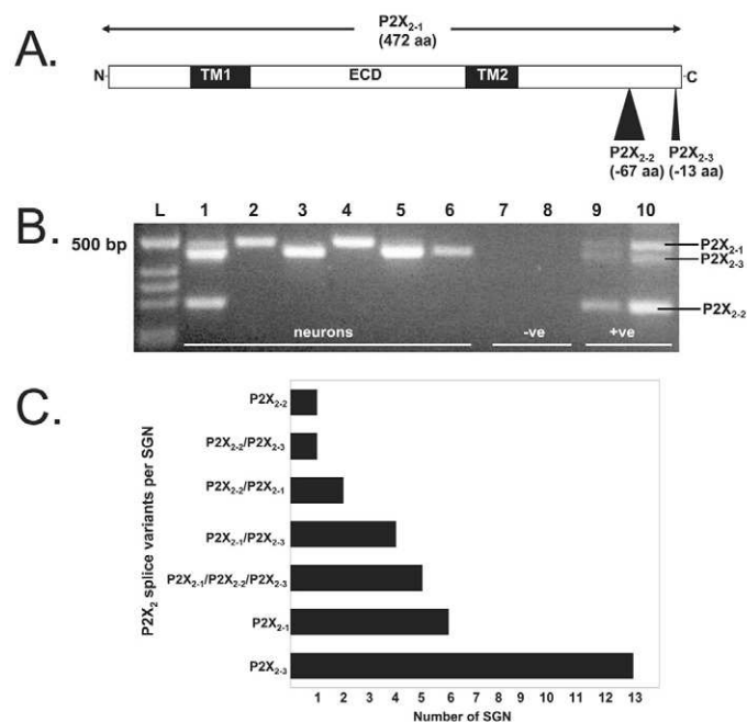
Fig. 4. Variation in expression of P2X 2 splice variants in SGN.
