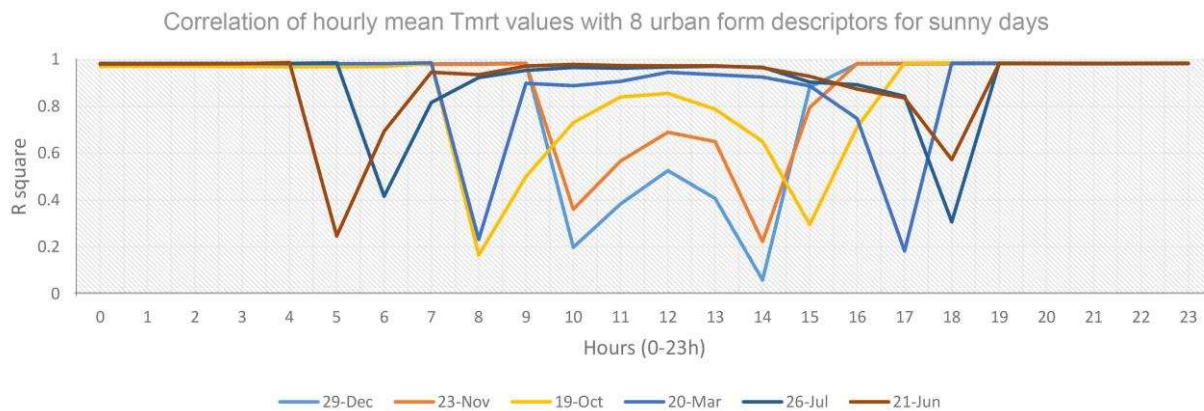
Figure 6: Correlation of hourly mean T_{mrt} values with 8 urban form descriptors on the sunny studied days.
