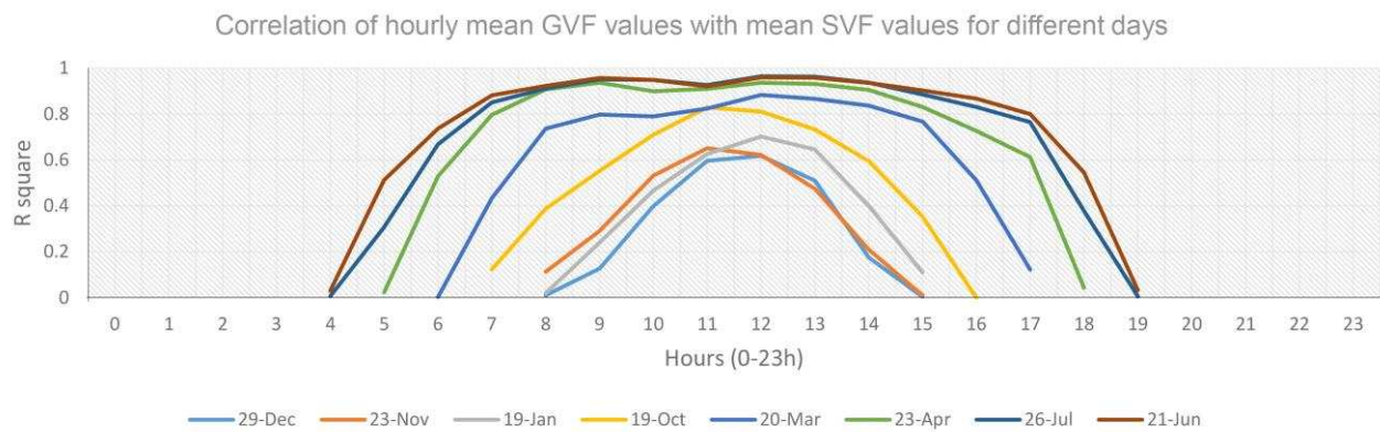
Figure 3: Correlation of hourly mean ground view factor (mean shadow fractions on ground) with mean sky view factor for the 8 days studied.
