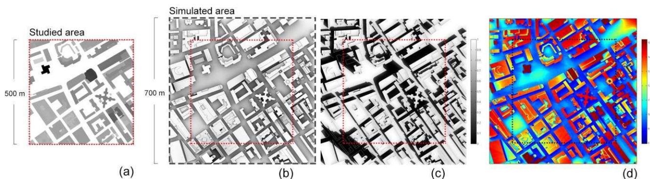
Figure 2: Square in central London (highlighted in Fig. 1): a) square's DEM, b) SVF values map, c) shadow pattern at 9am on 23 April (GVF) and d) T_{mrt} values map at 9am on 23 April (cloudy hour).
