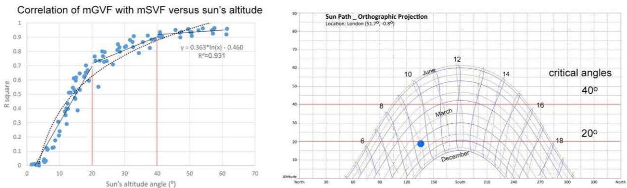
Figure 4: Left, correlation between mean ground view factor and mean sky view factor -expressed by R^2 - plotted against sun's altitude. Right, the sun path for London's location in orthographic projection. The crucial sun's altitude angles of 20° and 40° are highlighted by red lines.
