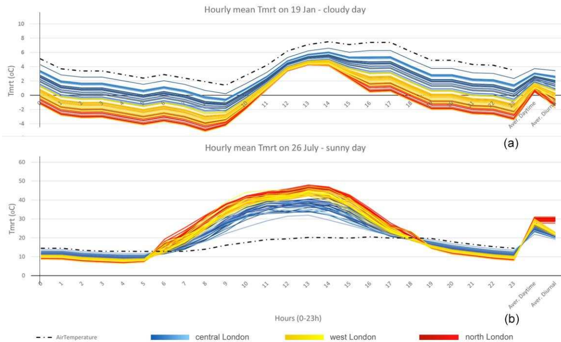
Figure 5: Hourly mean T_{mrt} values in outdoor space of 72 squares, (a) on a cloudy day and (b) on a sunny day
