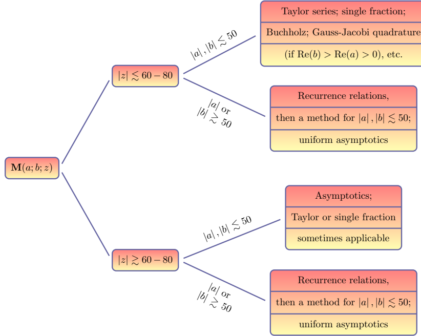
Figure 3.2: Summary of recommended methods for computing \mathbf{M} for different regions of a , b , and z .
