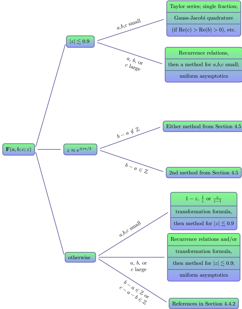
Figure 4.4: Summary of recommended methods for computing F for different values of the parameters a, b, and c and the variable z .
