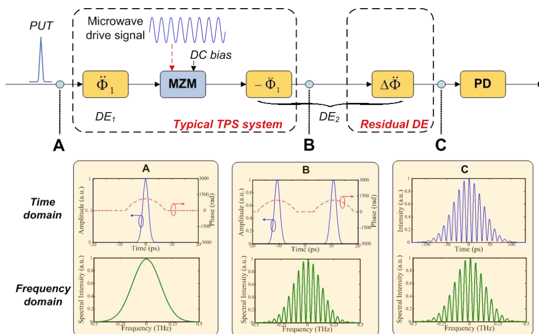
Figure 4. An alternative real-time spectral interferometry system for complete pulse characterization based on unbalanced temporal pulse shaping (UB-TPS). PUT: pulse under test, DE: dispersive element, PD: photodetector. [65].
