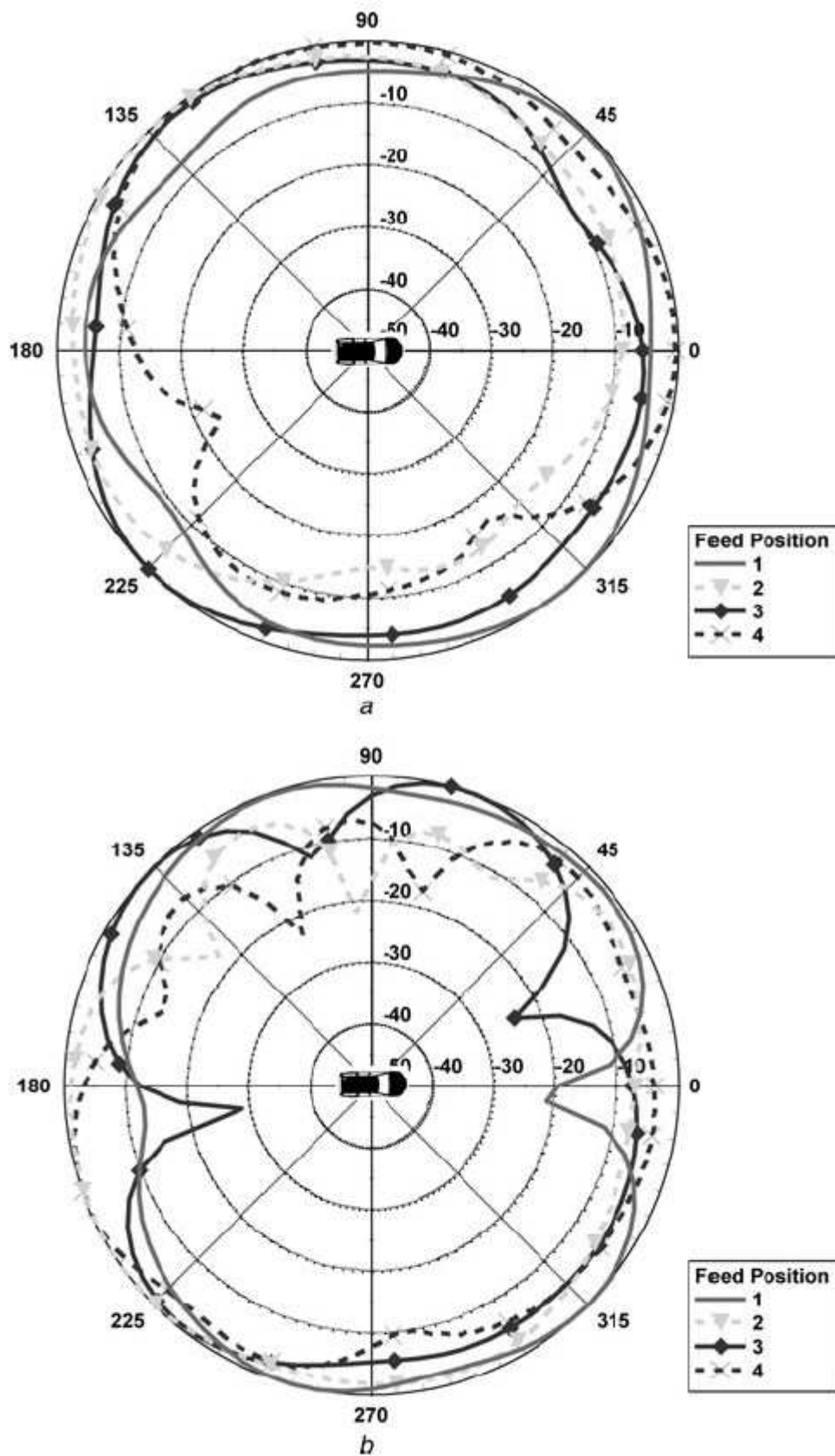
Fig. 8 Radiation pattern for various feed positions at 90 MHz a Vertical polarisation b Horizontal polarisation
