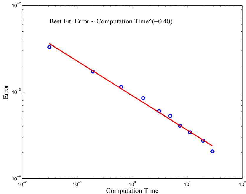
Figure 3: Convergence with non-equidistant discretization and the state-dependent drift \mu^L(t, S(t)) . The y-axis reports the absolute error |V_i - \hat{V}| of the value function V(t = 0, s = 15, x = 0, y = 0) . The benchmark \hat{V} = -0.9018 has been obtained by using N = 420 , and V_i 's are the results with N = 20 + i \times 20 , i = 0, 1, \dots, 9 .
