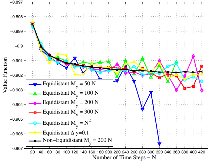
Figure 2: Value functions at initial time versus the number of time steps N with the state-dependent drift \mu^L(t, S(t)) , where N = 20 + i \times 20 , i = 0, 1, \dots, 20 . Other parameters are the same as in the base case.
