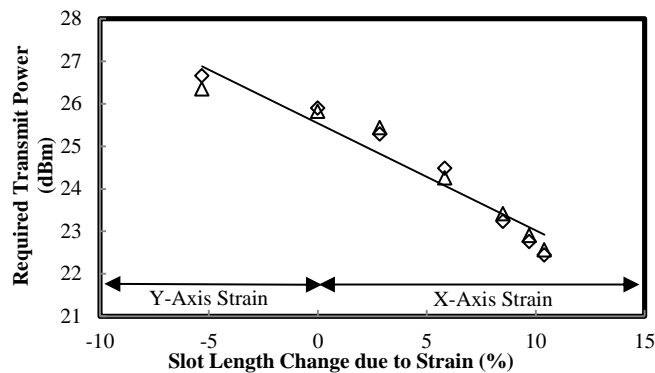
Fig. 6 Required transmitted power as function of slot length \Delta First Measurement, — trend line, \diamond measurement + 1 week.
