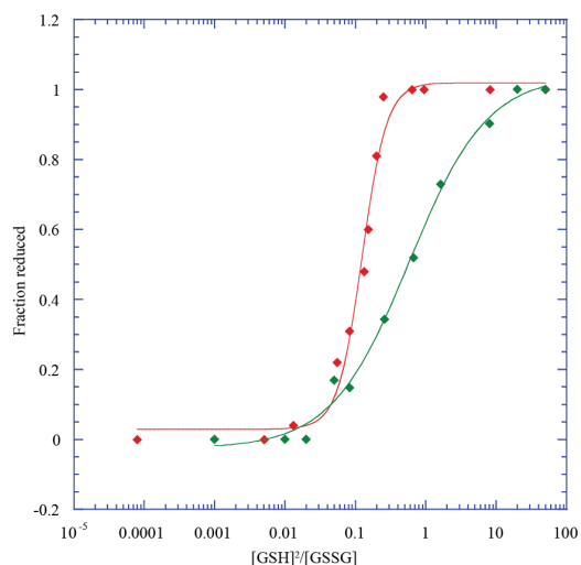
Fig. 2 Two fits shown using the Hill equation, PDI a , lysine 14 (green) with a redox potential of -144.43 \pm 0.34 mV and DsbA serine 43 (red) with a redox potential of -124.63 \pm 0.98 mV.
