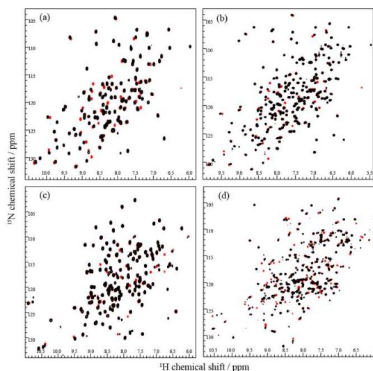
Fig. 1 ^{15} N HSQC spectra of (a) PDI a , (b) PDI ab , (c) ERp18 and (d) DsbA. Fully oxidised spectra are shown in red, and fully reduced spectra are shown in black.
