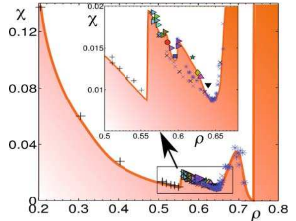
Fig. 5. ‘Granular temperature’ (compactivity \chi ) vs. packing fraction \rho . The symbols * refer to 25 numerical simulations of packings with 10 000 spheres generated by using the Jodrey-Tory algorithm [23].
