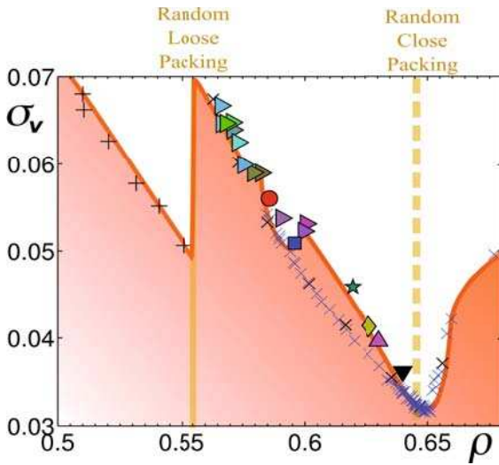
Fig. 3. Behavior of the standard deviation of the Voronoi volume fluctuations ( \sigma_v ) vs. packing fraction ( \rho ). Very sharp changes are observed at \rho \sim 0.555 and at \rho \sim 0.645 . Symbols are as in Figure 1.
